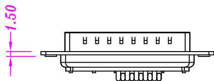
Plug Contact
