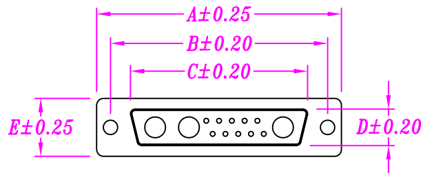
Plug Contact
