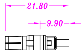
Plug Contact
