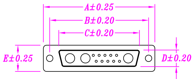
Plug Contact
