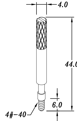
(STL-4*44-1)
