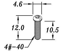
(STF-4*12.5)
