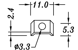
(SSW-4)
